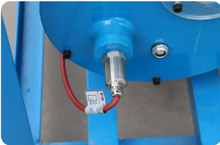
Hose leak detection device
